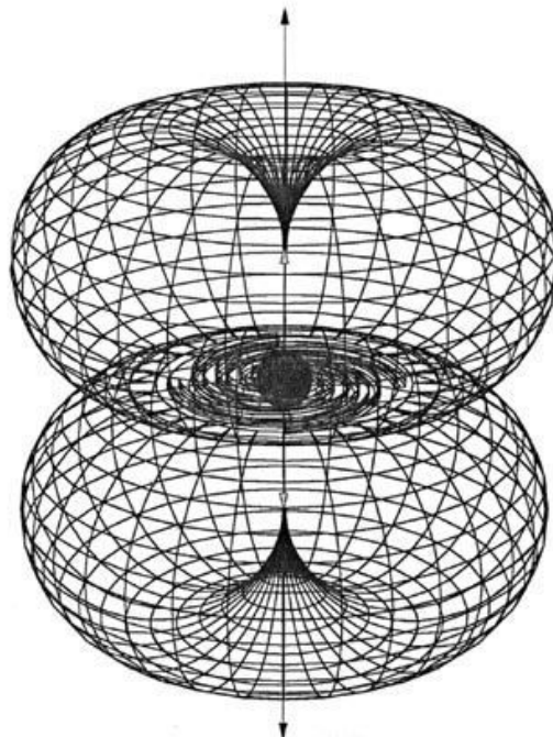
Figure 1. Galactic Singularity Engine: Origin of Life
